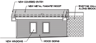
Brook (west) Elevation
