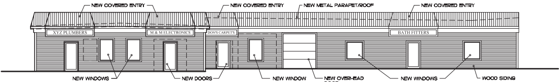
Elm Street (north) Elevation
