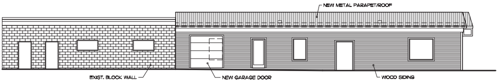
Alley (east) Elevation
