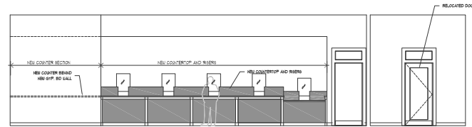
INTERIOR ELEVATION - TELLER LINE
